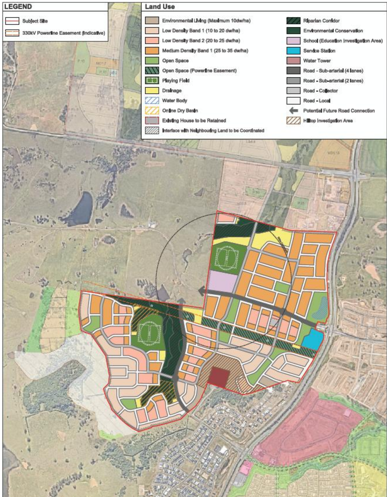
Figure 3 Indicative Layout Plan
